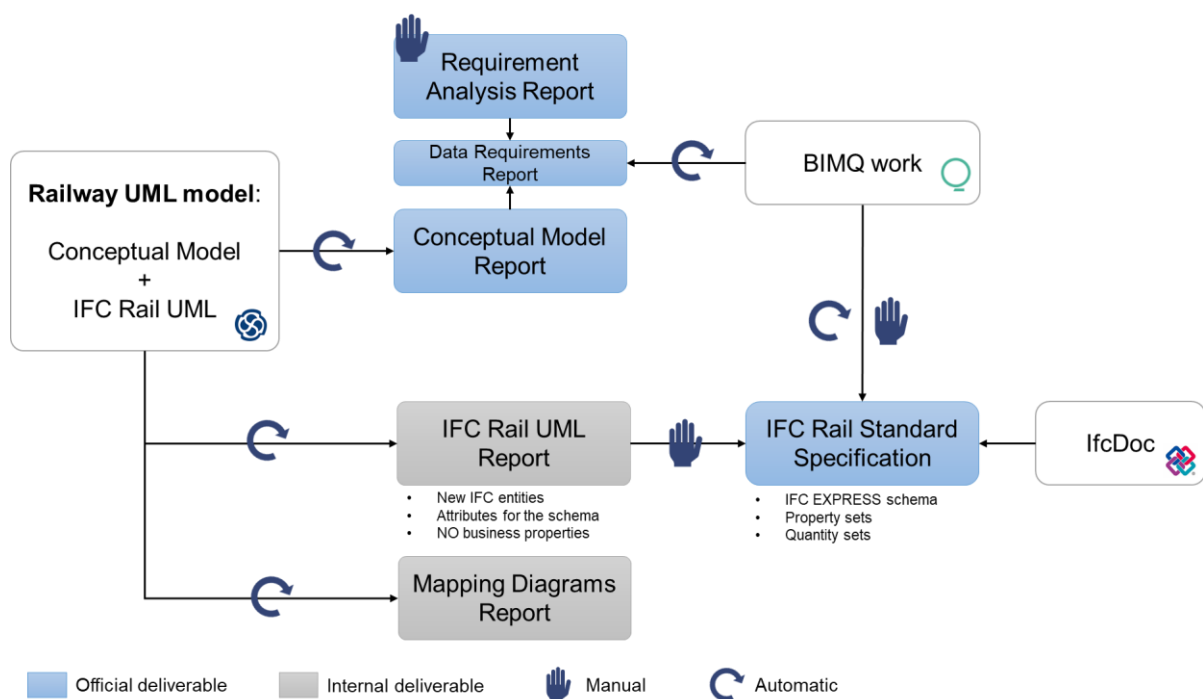
Figure 7 – Summary of the tool-chain
